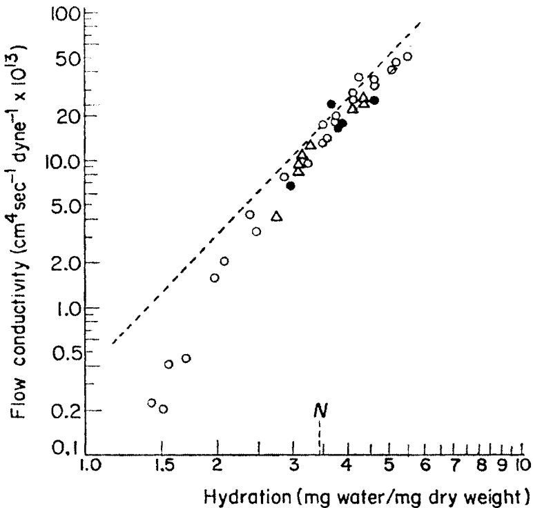
Figure 6 Flow conductivity versus hydration across the cornea. The symbols refer to measurements taken with (closed circles) and without (open circles) Descemet's membrane in 0.9% NaCl, or without Descemet's membrane in distilled water (triangles). The broken line represents the flow conductivity versus hydration relationship for flow along the cornea. N is the normal corneal hydration. From Hedbys & Mishima (144).
